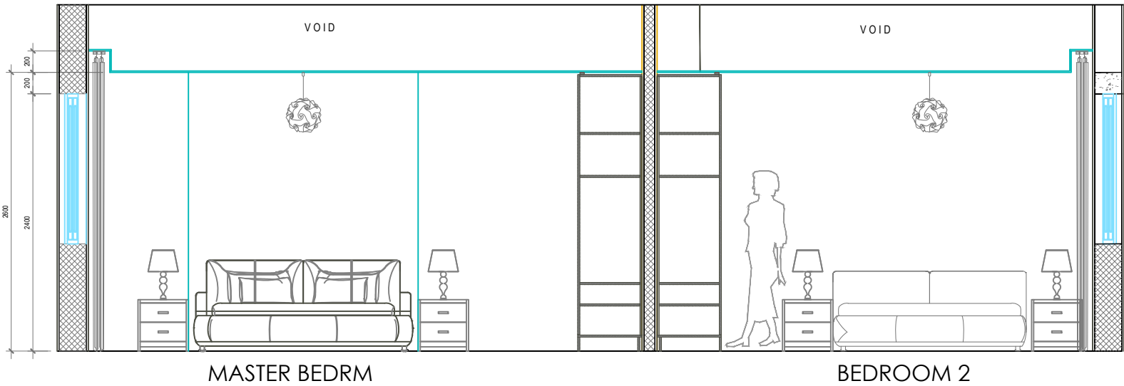
1 SE-01 MODEL C DUPLEX - FIRST FLOOR SECTION - ELEVATION SCALE 1:50
