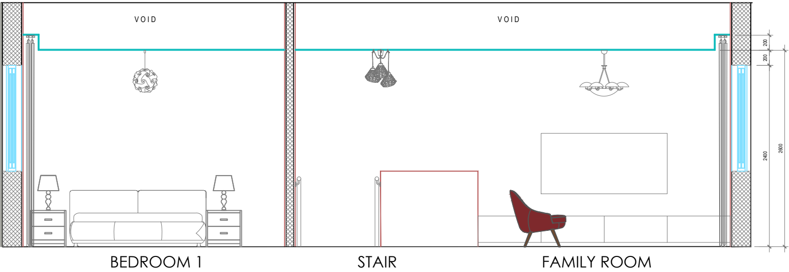
2 SE-01 MODEL C DUPLEX - FIRST FLOOR SECTION - ELEVATION SCALE 1:50
