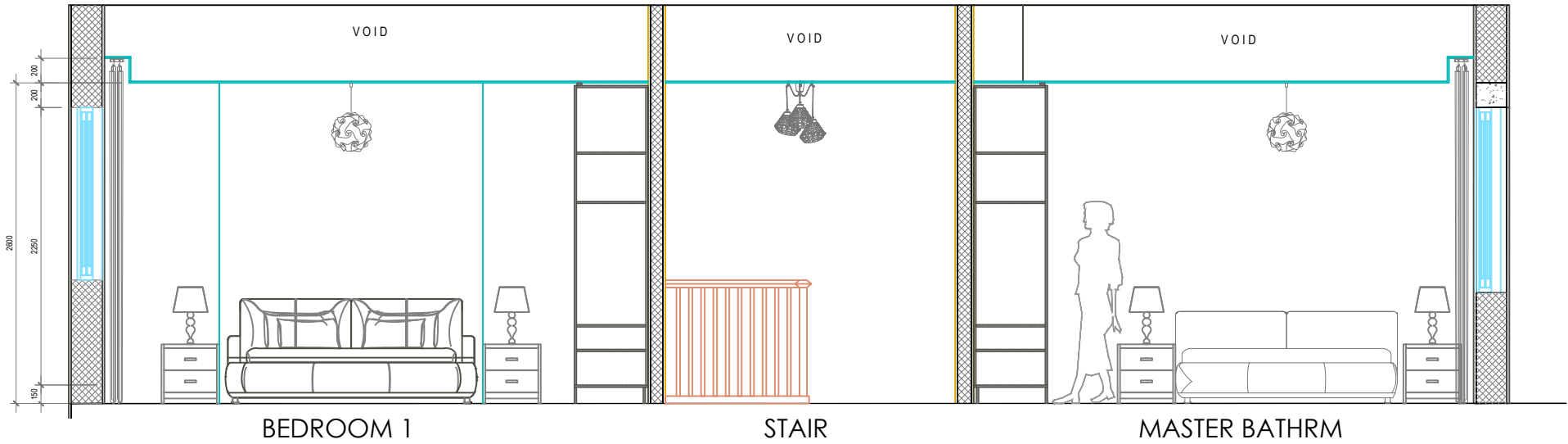
1 SE-01 MODEL B DUPLEX - FIRST FLOOR SECTION - ELEVATION SCALE 1:50
