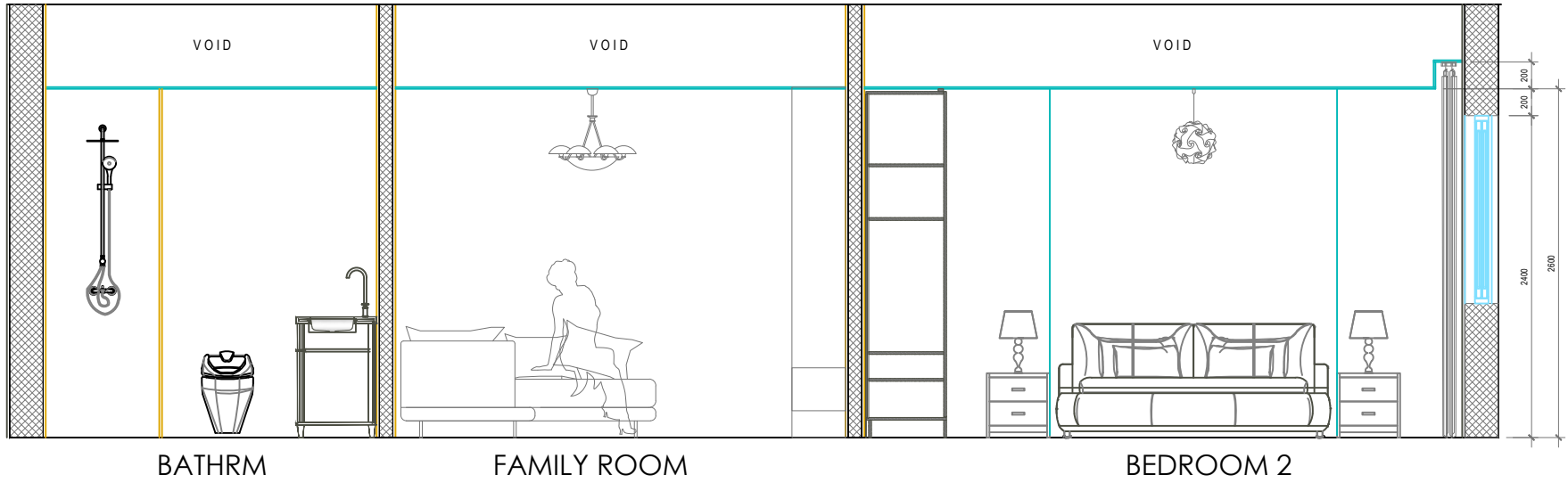
2 SE-01 MODEL B DUPLEX - FIRST FLOOR SECTION - ELEVATION SCALE 1:50
